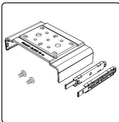
Slide Mount Bracket, Guide Rails and Screws
